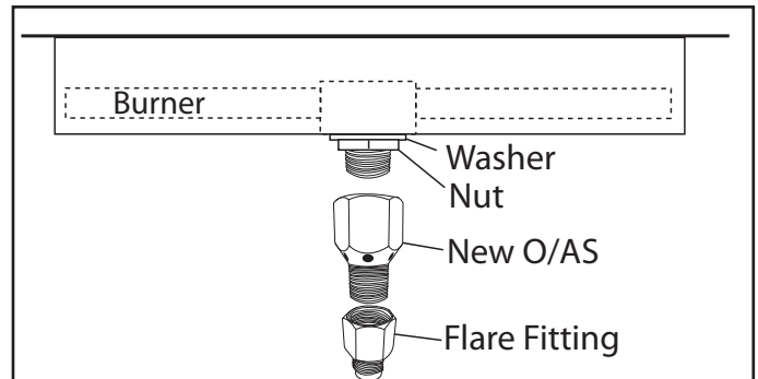
Fig. 2 Installing new OAS
